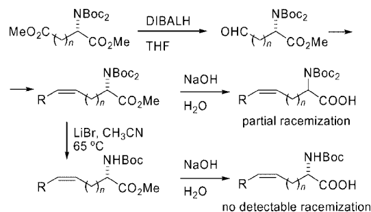
Scheme 1. Selectivity and modification in reactivity in N,N -di-Boc \alpha -amino diesters.
